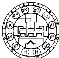
BOTTOM VIEW BUTTON 12 PIN BASE 12BQ
